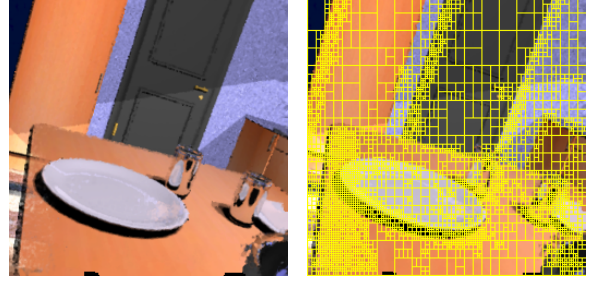
Figure 3: A reconstructed image and an overlay showing the tiling used by the sampler at that moment in time. Note the finer tilings over object edges and occlusions.
